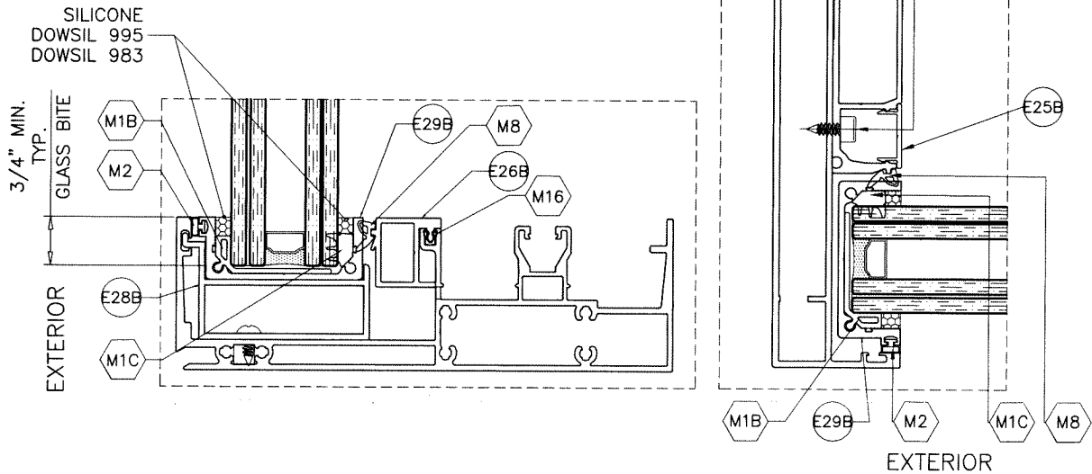
GLAZING DETAIL AT FIXED PANEL 1-1/2" OVERALL INSUL. DOUBLE LAM. GLASS
