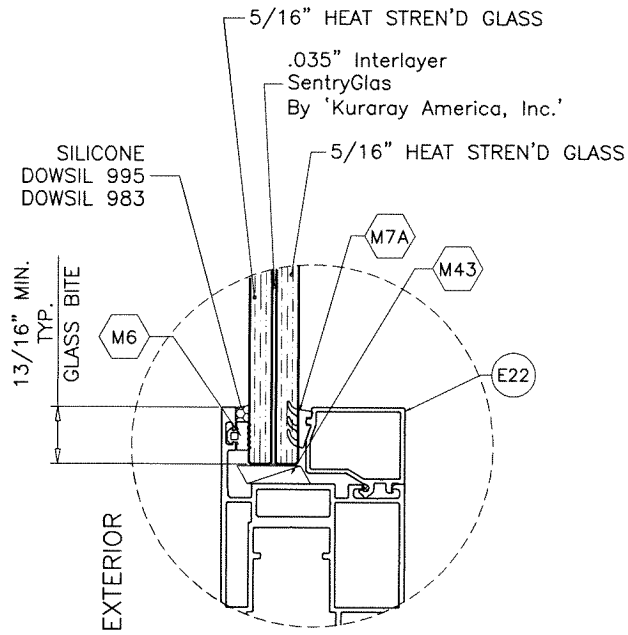
GLASS TYPE 'A1' 11/16" LAM. GLASS GLAZING DETAIL AT MOVING PANEL
