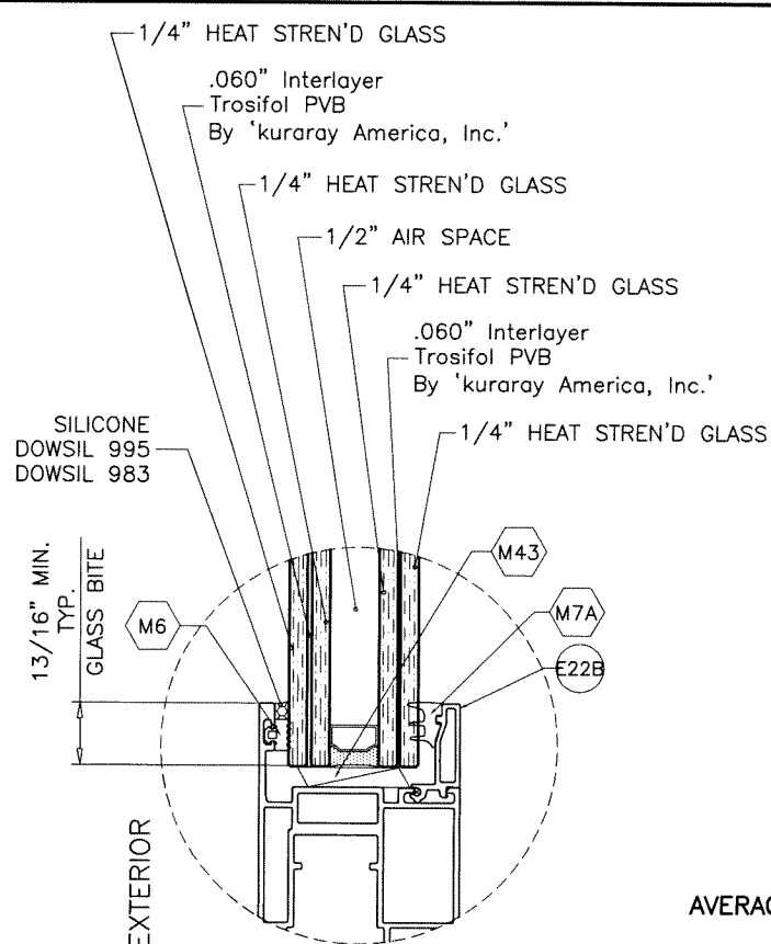
GLASS TYPE 'F' 1-1/2" OVERALL INSUL. DOUBLE LAM. GLASS GLAZING DETAIL AT MOVING PANEL
