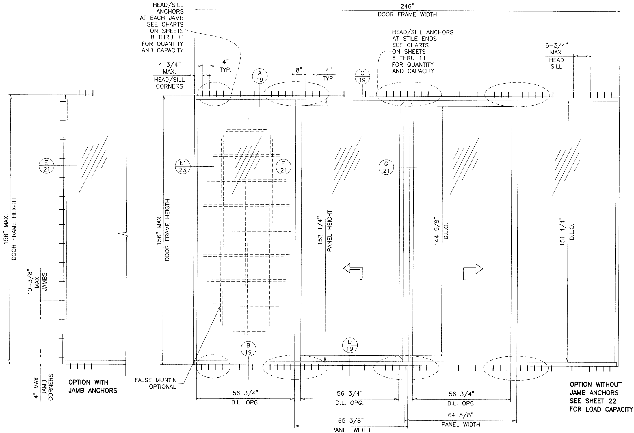
TYPICAL ELEVATIONS (OX-XO) WITHOUT HEAD RECEPTOR
